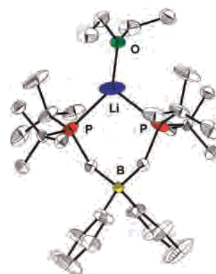
Figure 6. A 50% displacement ellipsoid representation of [\text{Ph}_2\text{B}(\text{CH}_2\text{P}^t\text{Bu}_2)_2][\text{Li}(\text{OEt})_2] ( 37 [Li]). Hydrogen atoms and disordered positions are omitted for clarity. Selected interatomic distances (Å) and angles (deg): P–Li, 2.485(4); Li–O, 1.926(8); B–Li, 4.092(8); P–Li–O, 121.31(14); P–Li–P, 99.5(2).
