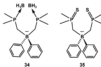
Figure 2. Protected alkylbis(phosphino)borates.
