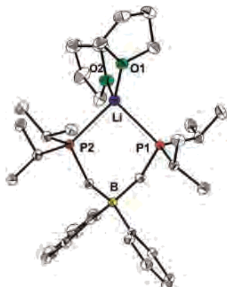
Figure 5. A 50% displacement ellipsoid representation of [\text{Ph}_2\text{B}(\text{CH}_2\text{P}^t\text{Bu}_2)_2][\text{Li}(\text{THF})_2] ( 36 [Li]). Hydrogen atoms are omitted for clarity. Selected interatomic distances (Å) and angles (deg): Li–P1, 2.608(3); Li–P2, 2.596(3); Li–O1, 1.962(3); Li–O2, 1.928(3); Li–B, 4.197(3); P1–Li–P2, 91.07(9); O1–Li–O2, 104.93(14); P1–Li–O1, 116.77(13); P2–Li–O2, 107.46(13); P1–Li–O2, 112.56(13); P2–Li–O1, 123.68(13).
