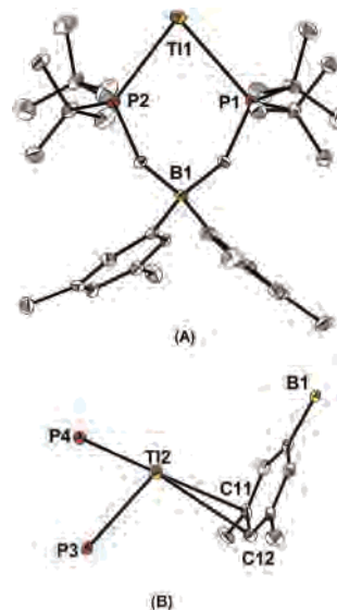
Figure 7. (A) A 50% displacement ellipsoid representation of [(m,m\text{-}(\text{CH}_3)_2\text{Ph})_2\text{B}(\text{CH}_2\text{P}^t\text{Bu}_2)_2][\text{Tl}] ( 38 [Tl]). Hydrogen atoms and second molecule of the asymmetric unit are omitted for clarity. Selected interatomic distances (Å) and angles (deg): P1–Tl1, 2.9919(12); P2–Tl1, 2.9426(11); B1–Tl1, 4.786(5); P1–Tl1–P2, 78.75(3). (B) Intermolecular interactions within the asymmetric unit, emphasizing the thallium coordination sphere. Selected interatomic distances (Å) and angles (deg): P3–Tl2, 2.9788(12); P4–Tl2, 2.9406(11); C11–Tl2, 3.388(4); C12–Tl2, 3.353(4).
